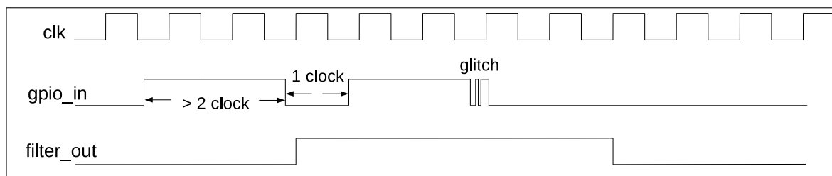
Figure 5.4-2. GPIO Filter Timing of GPIO Input Signals
