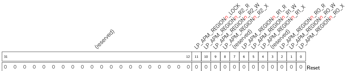
Register 13.32. LP_APM_REGION n _ATTR_REG ( n : 0-7) (0x000C+0xC* n )
