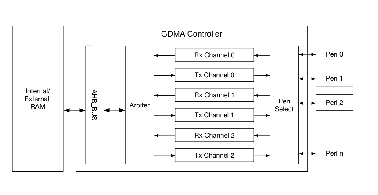
Figure 3.3-1. GDMA controller Architecture
