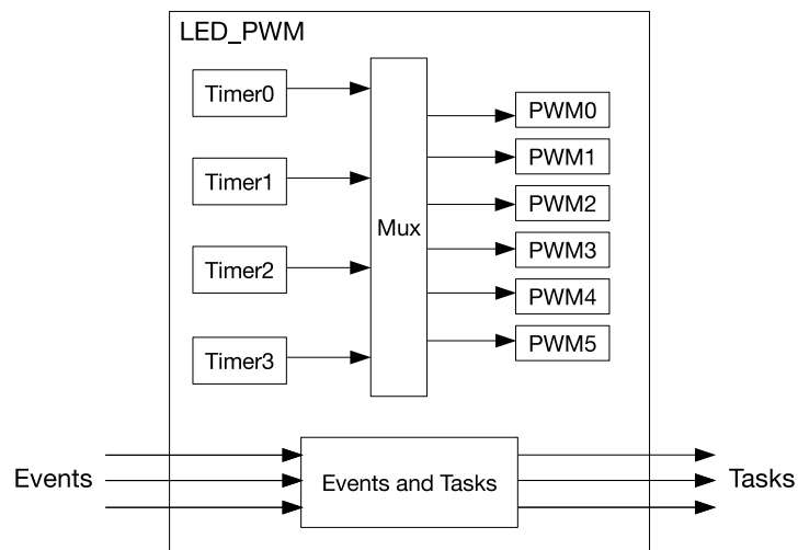
Figure 30.3-1. LED PWM Architecture
