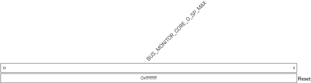
Register 14.28. BUS_MONITOR_CORE_O_SP_MAX_REG (0x003C)
