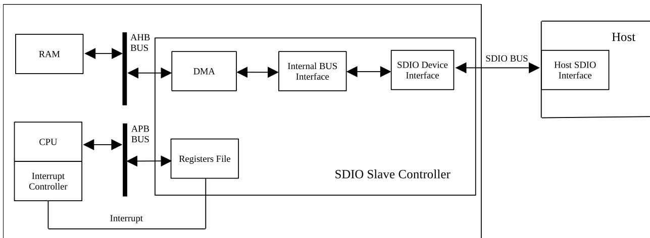
Figure 29.3-1. SDIO Slave Block Diagram
