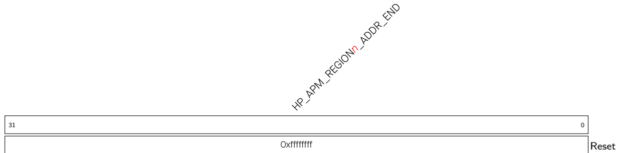
Register 13.3. HP_APM_REGION n _ADDR_END_REG ( n : 0-15) (0x0008+0xC* n )
