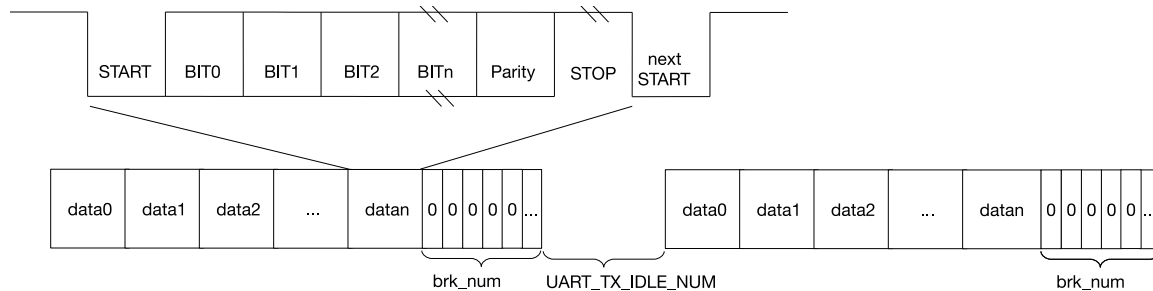
Figure 25.4-3. Structure of UART Data Frame
