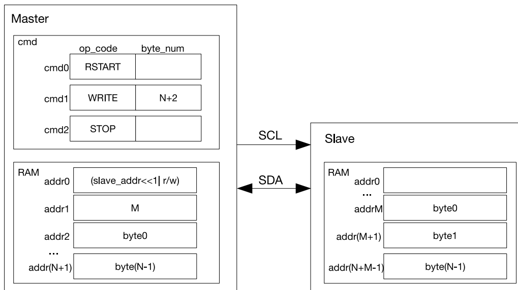
Figure 26.7-3. I2C master Writing to I2C slave with Two 7-bit Addresses
