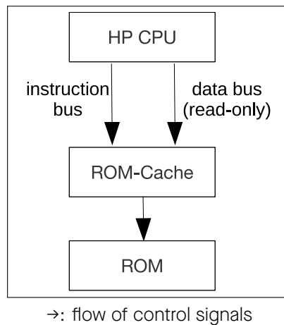
Figure 4.3-2. ROM-Cache Structure
