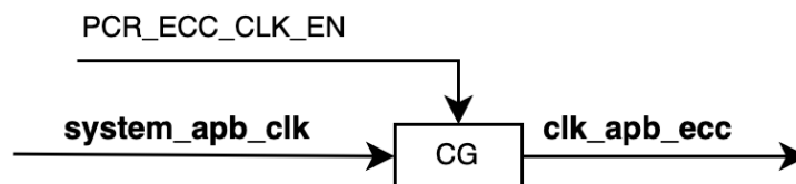
Figure 17.4-2. clk_apb_ecc Diagram
