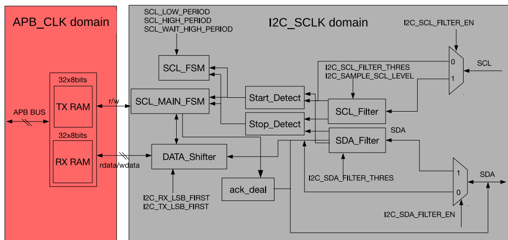
Figure 26.3-2. I2C Slave Architecture
