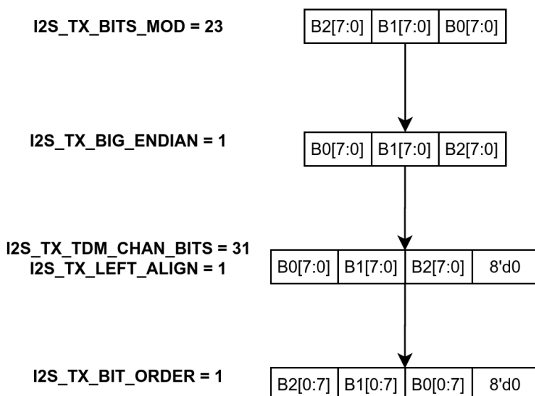
Figure 27.9-1. TX Data Format Control
