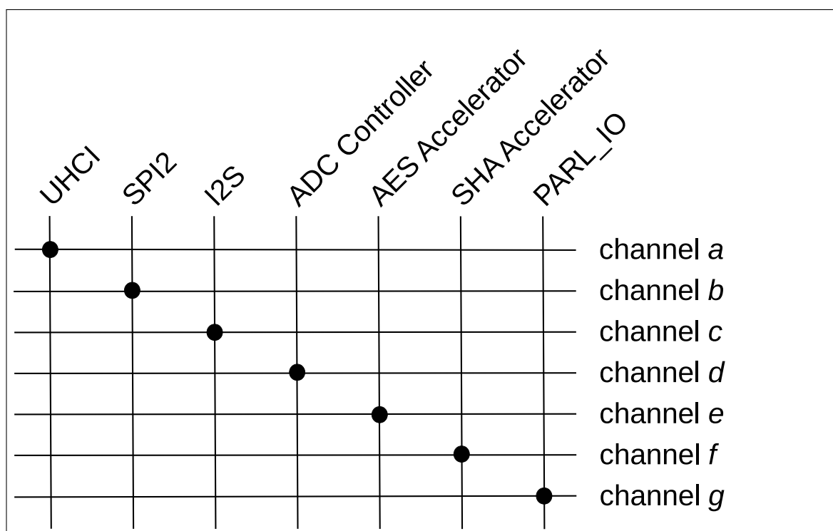
Figure 4.3-4. Modules/peripherals that can work with GDMA
