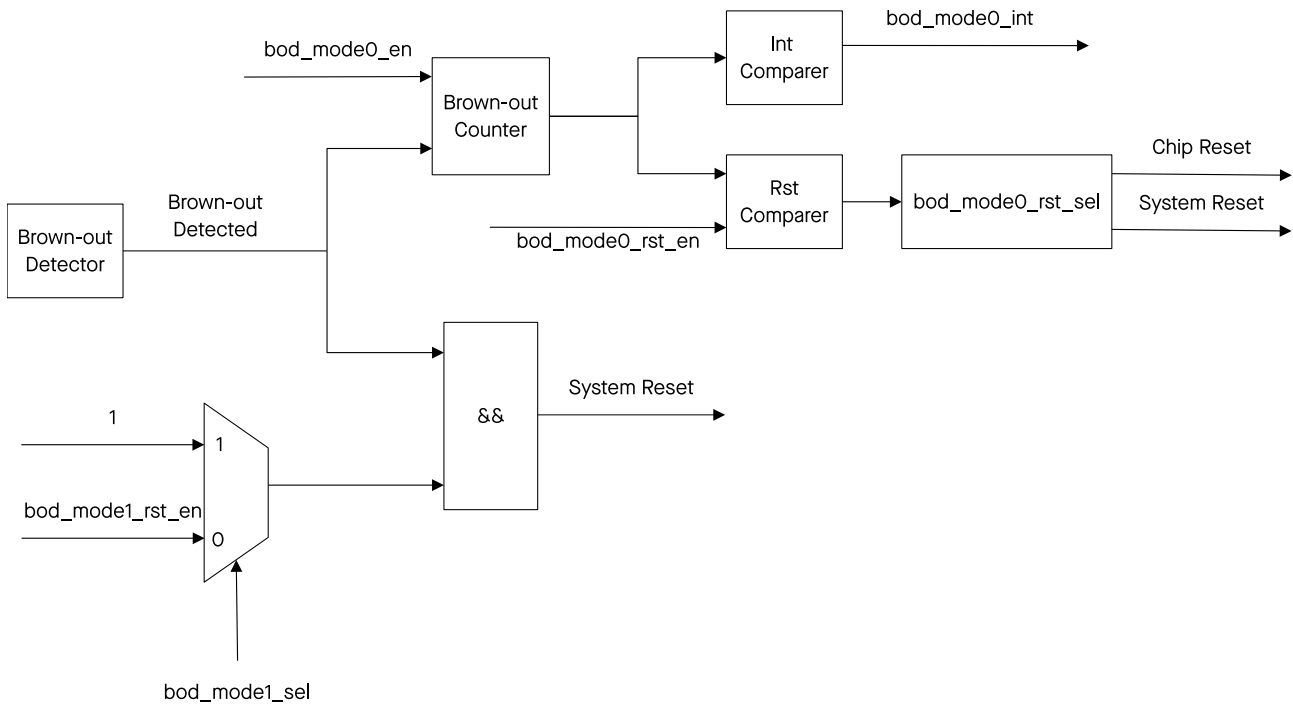
Figure 15.3-2. Brown-out Reset Workflow
