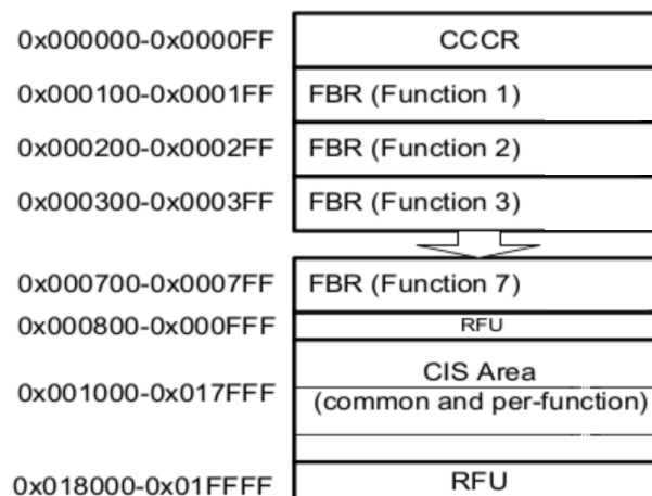
Figure 29.5-3. Function 0 Address Space
