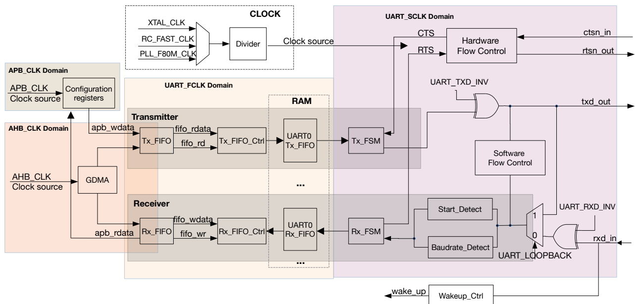
Figure 25.3-1. UART Structure
