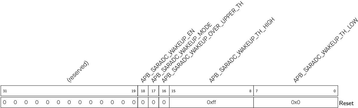
Register 35.3. APB_TSENS_WAKE_REG (0x0064)
