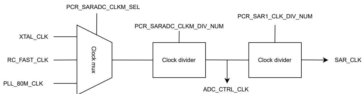
Figure 36.5-1. SAR ADC Clock Structure
