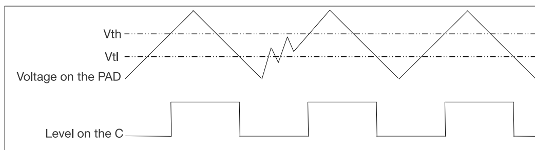
Figure 5.10-2. Example of Level Flip on the Chip Pad — Hysteresis Function Enabled
