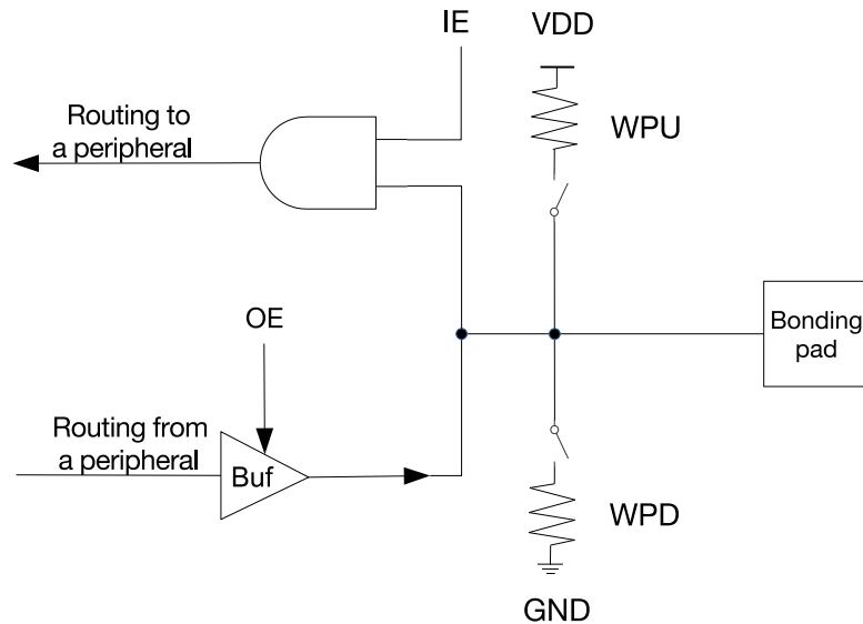
Figure 5.3-2. Internal Structure of a Pad
