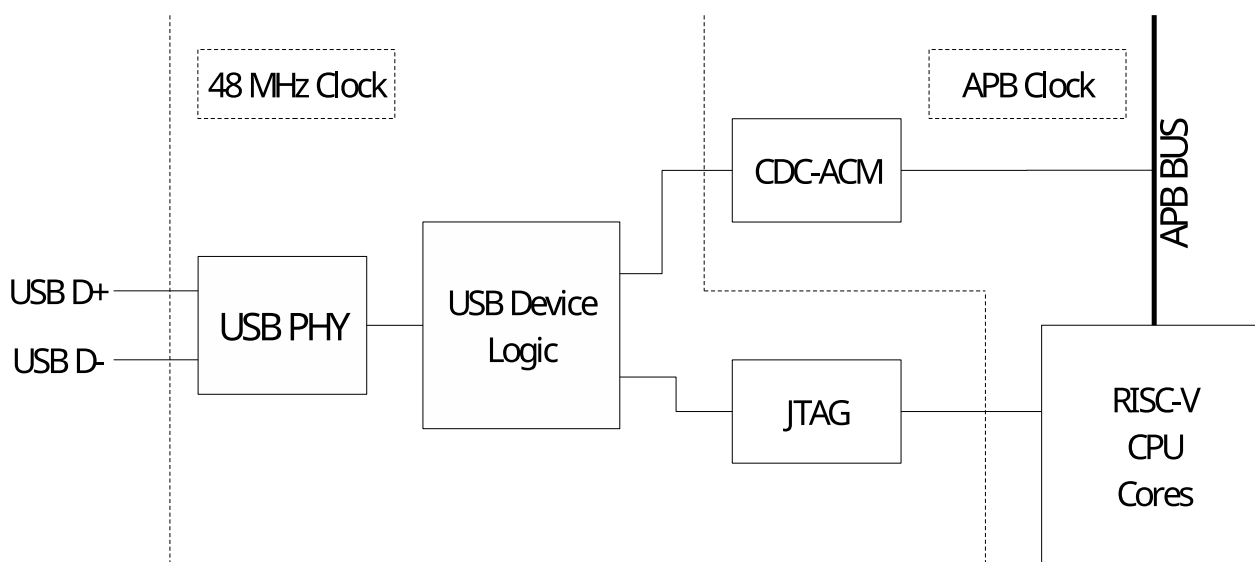
Figure 28.2-1. USB Serial/JTAG High Level Diagram
