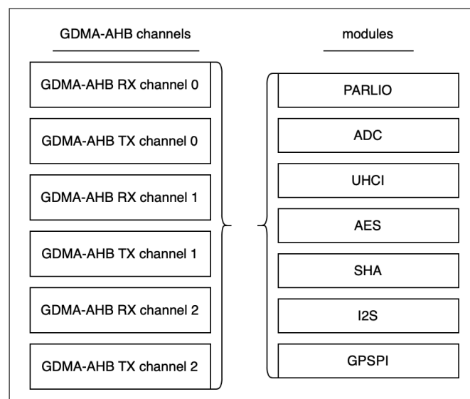
Figure 3.1-1. Modules that Share GDMA Channels
