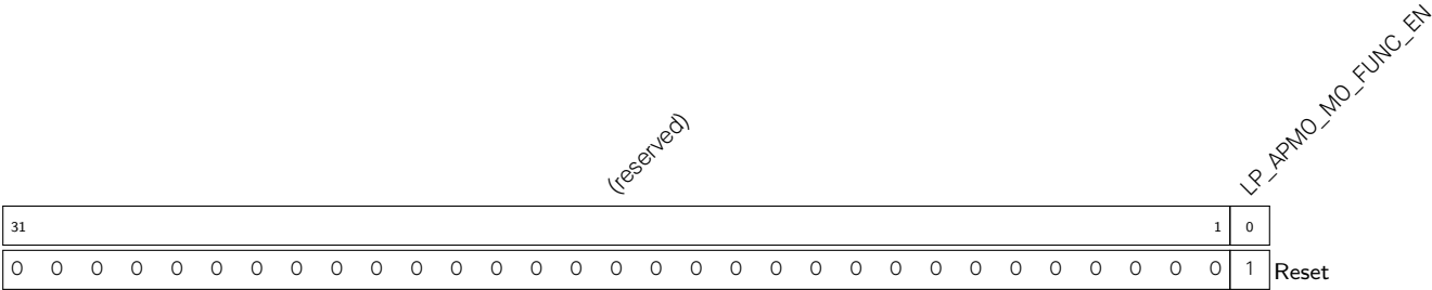
Register 13.49. LP_APMO_FUNC_CTRL_REG (0x00C4)
