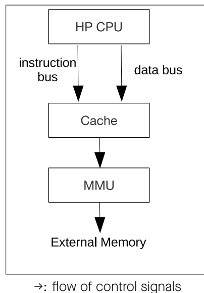
Figure 4.3-3. Cache Structure
