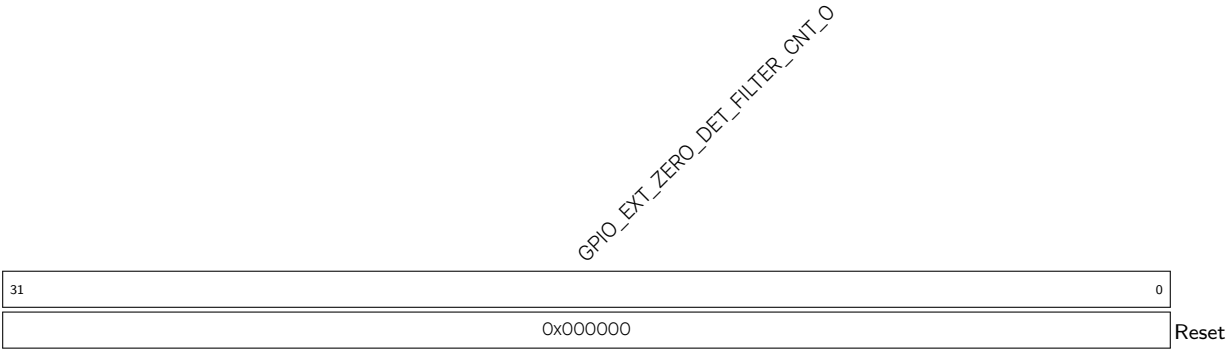
Register 5.29. GPIO_EXT_PAD_COMP_FILTER_O_REG (0x005C)
