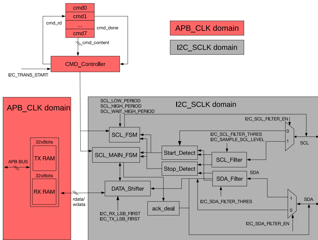
Figure 26.3-1. I2C Master Architecture
