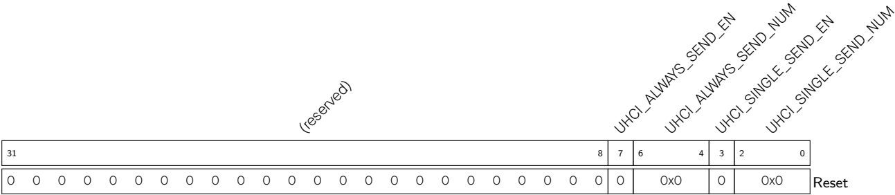
Register 25.75. UHCI_QUICK_SENT_REG (0x0030)
