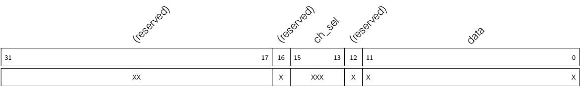
Figure 36.5-8. DMA Data Format
