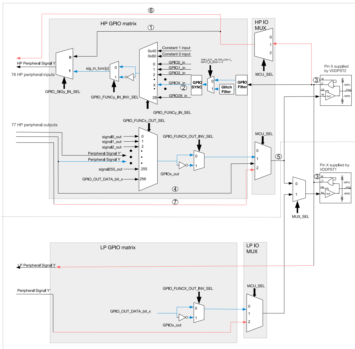
Figure 5.3-1. Architecture of HP GPIO Matrix, HP IO MUX, LP GPIO Matrix, and LP IO MUX
