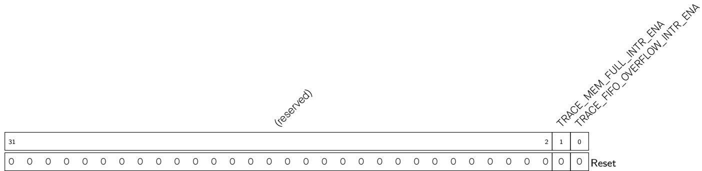
Register 1.6. TRACE_INTR_ENA_REG (0x0014)
