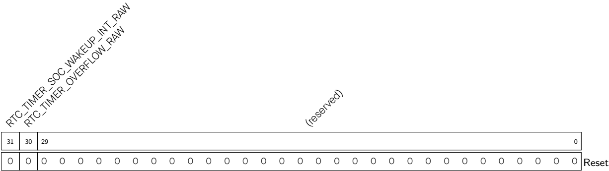
Register 12.10. RTC_TIMER_INT_RAW_REG (0x0028)
