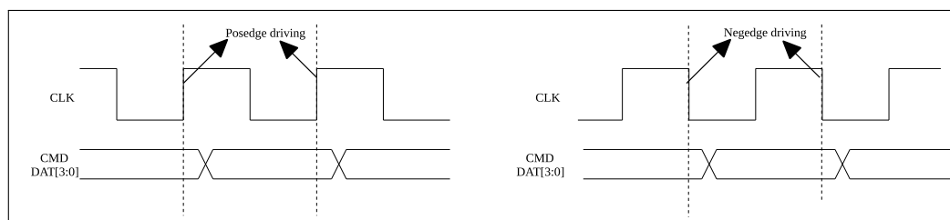
Figure 29.5-9. Output Timing Diagram
