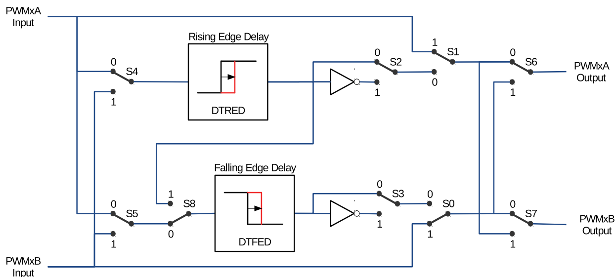
Figure 31.3-21. Options for Setting up the Dead Time Generator Module
