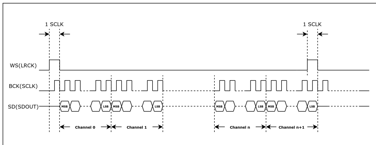
Figure 27.5-3. TDM PCM Standard Timing Diagram
