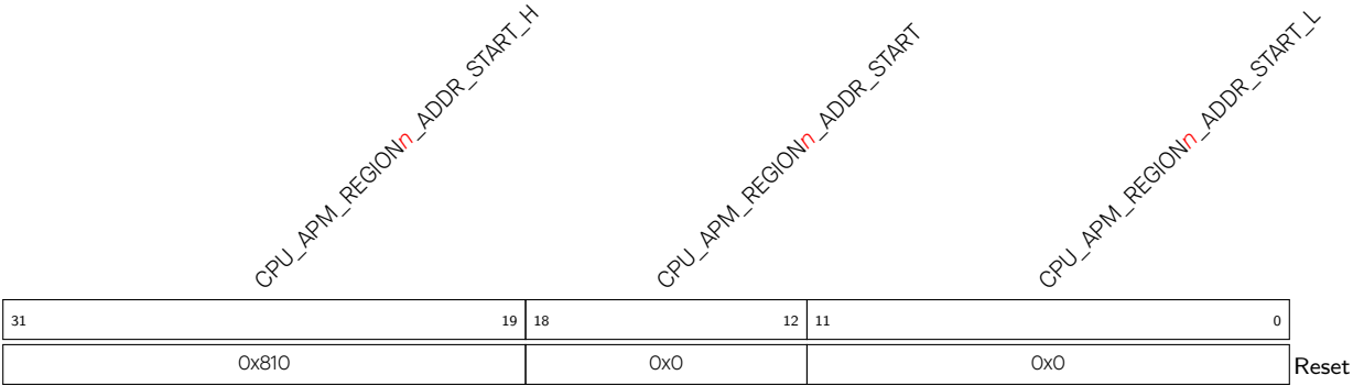
Register 13.58. CPU_APM_REGION n _ADDR_START_REG ( n : 0-7) (0x0004+0xC* n )
