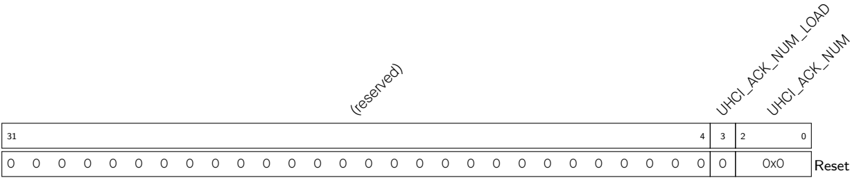
Register 25.74. UHCI_ACK_NUM_REG (0x0028)
