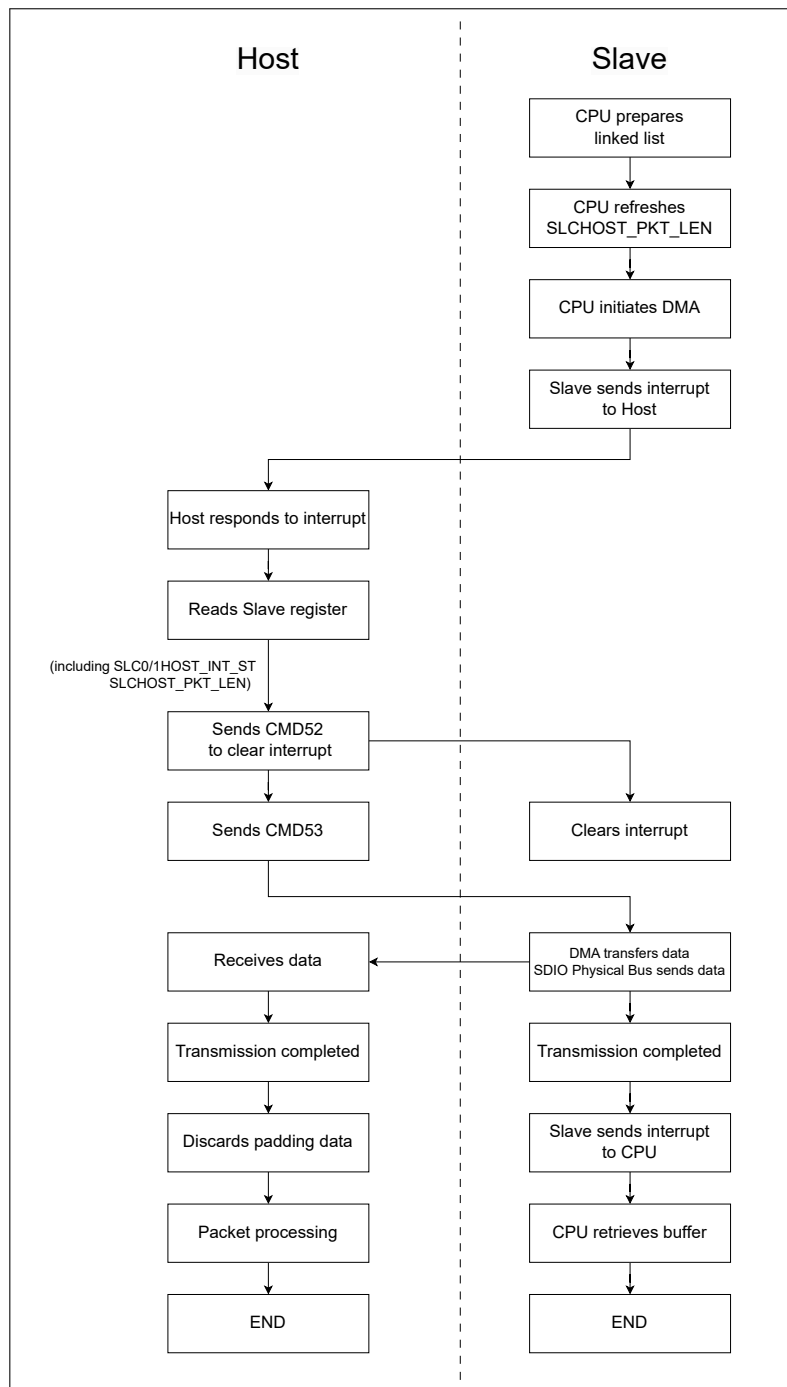
Figure 29.7-1. Procedure of Slave Sending Packets to Host
