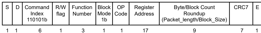
Figure 29.5-2. CMD53 Content
