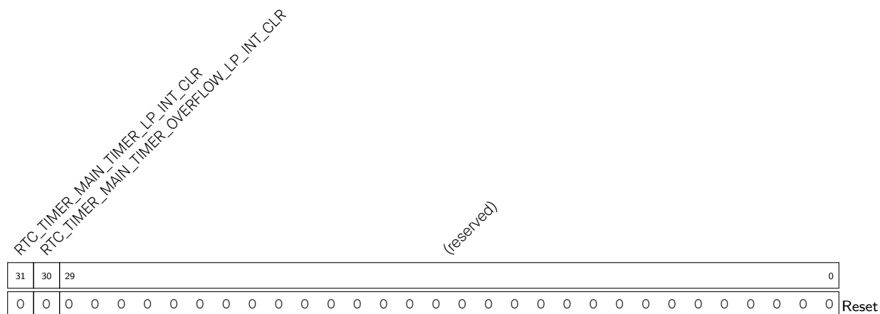
Register 12.17. RTC_TIMER_LP_INT_CLR_REG (0x0044)
