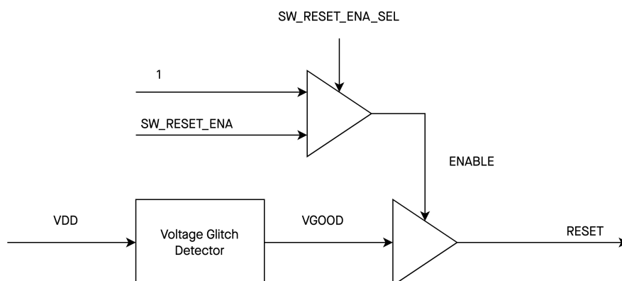
Figure 15.3-3. Structure of Voltage Glitch Detectors
