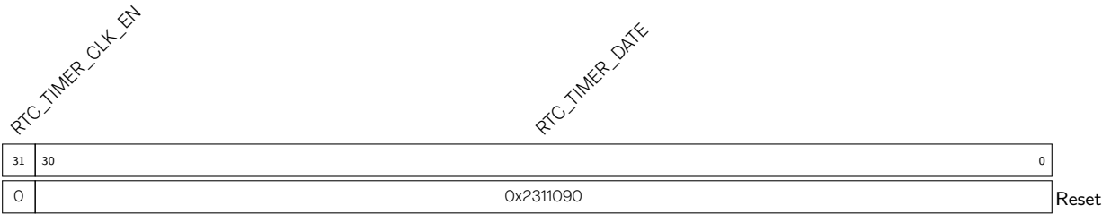
Register 12.18. RTC_TIMER_DATE_REG (0x03FC)
