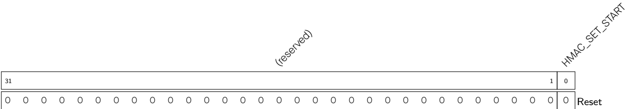
Register 18.1. HMAC_SET_START_REG (0x0040)
