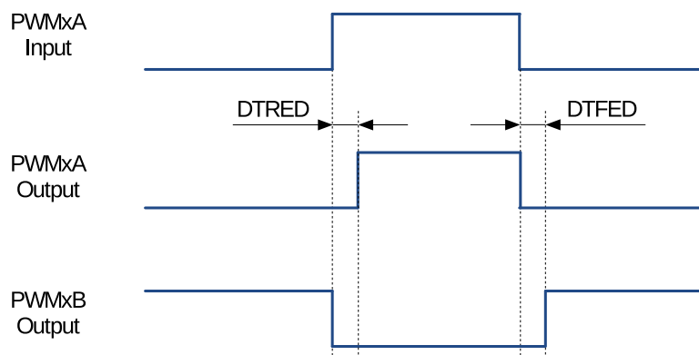
Figure 31.3-22. Active High Complementary (AHC) Dead Time Waveforms
