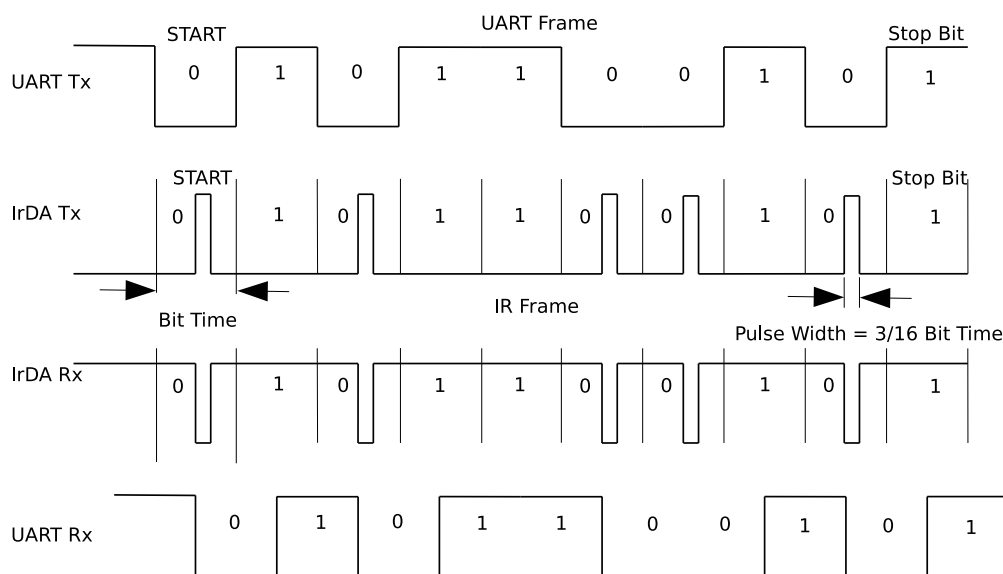
Figure 25.4-6. The Timing Diagram of Encoding and Decoding in SIR mode
