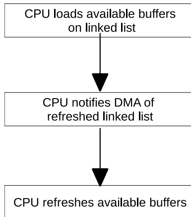
Figure 29.7-3. Loading Receiving Buffer
