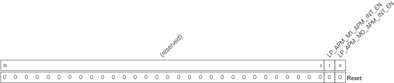
Register 13.42. LP_APM_INT_EN_REG (0x00E8)
