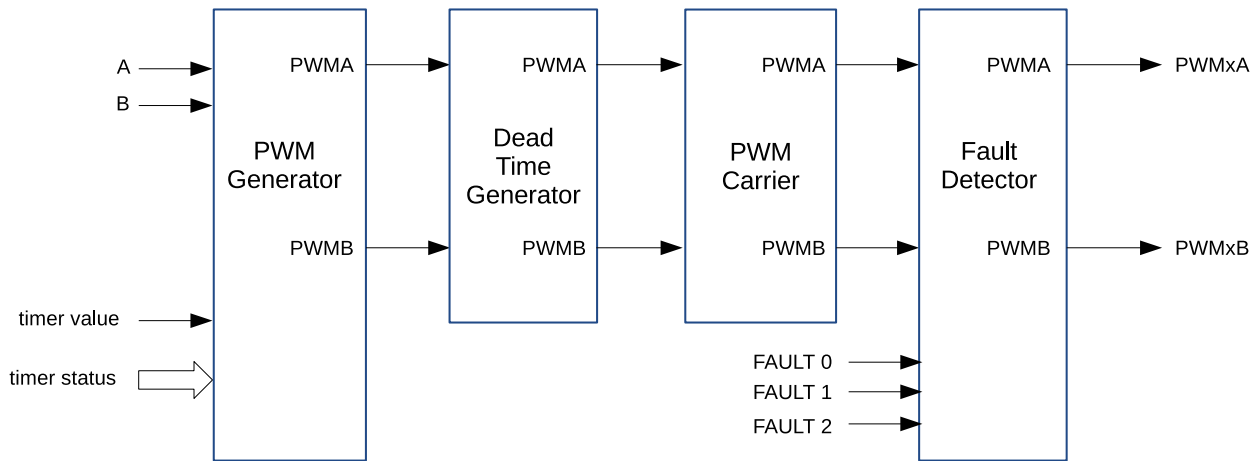
Figure 31.3-12. Block Diagram of A PWM Operator
