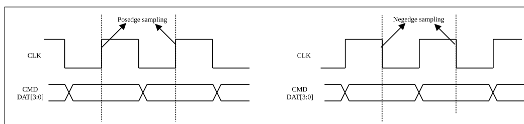
Figure 29.5-8. Sampling Timing Diagram
