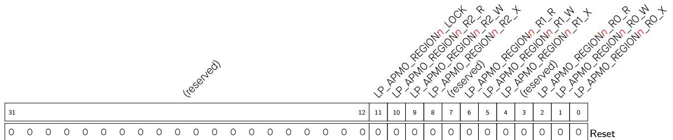
Register 13.48. LP_APMO_REGION n _ATTR_REG ( n : 0-7) (0x000C+0xC* n )
