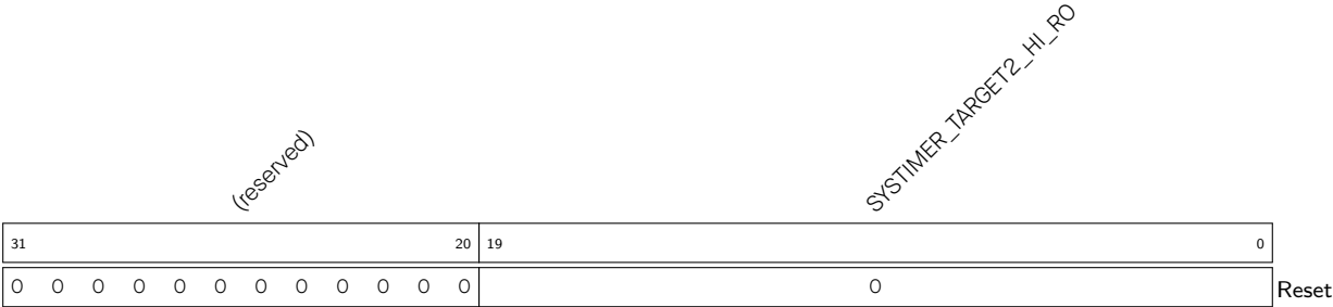
Register 9.35. SYSTIMER_REAL_TARGET2_HI_REG (0x0088)
