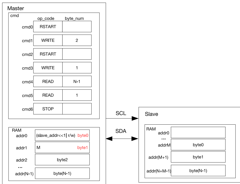
Figure 26.7-7. I2C master Reading N Bytes of Data from addrM of I2C slave with a 7-bit Address
