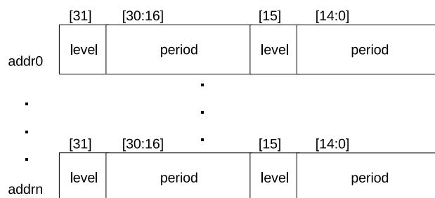
Figure 32.3-2. Format of Pulse Code in RAM
