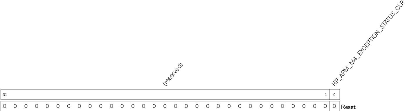
Register 13.23. HP_APM_M4_STATUS_CLR_REG (0x010C)
