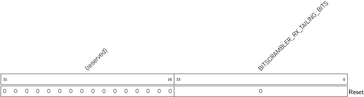
Register 34.10. BITSCRAMBLER_RX_TAILING_BITS_REG (0x0024)
