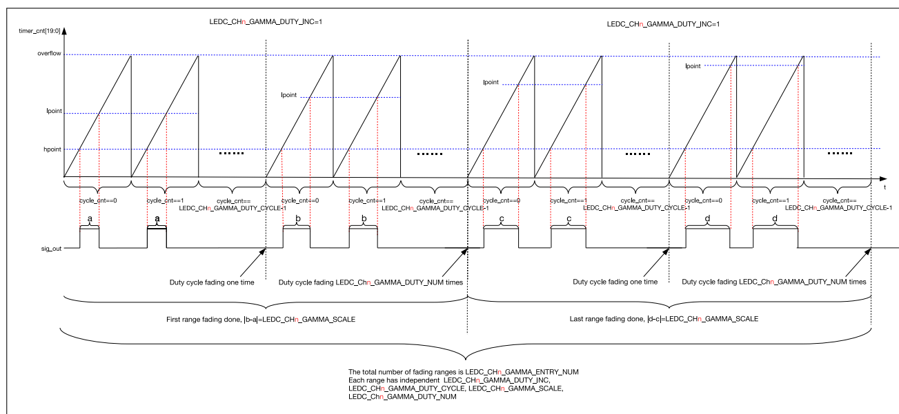
Figure 30.4-5. Output Signal of Gamma Curve Fading
