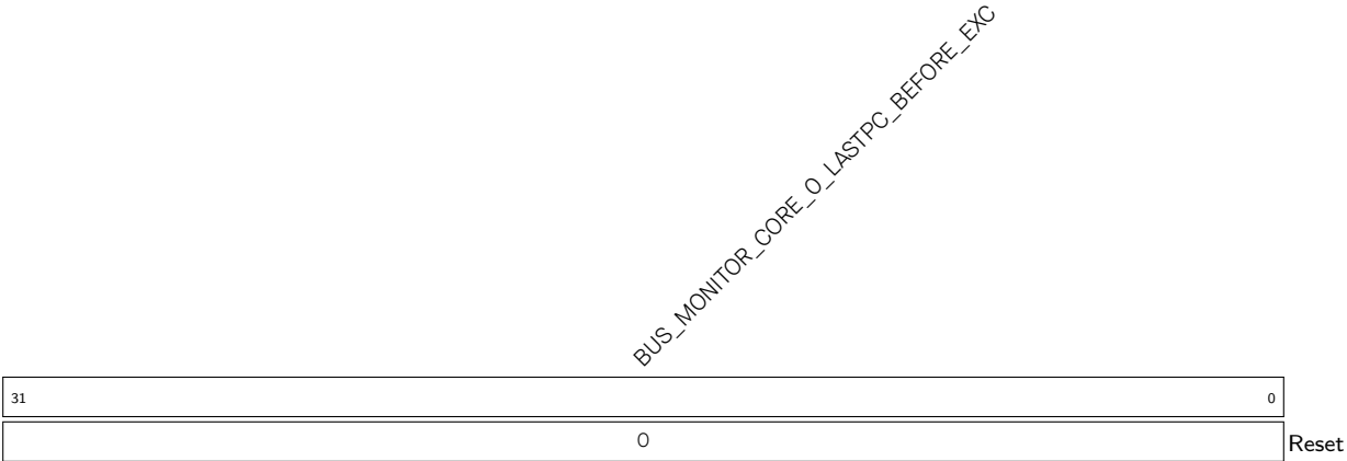
Register 14.36. BUS_MONITOR_CORE_O_LASTPC_BEFORE_EXCEPTION_REG (0x0070)
