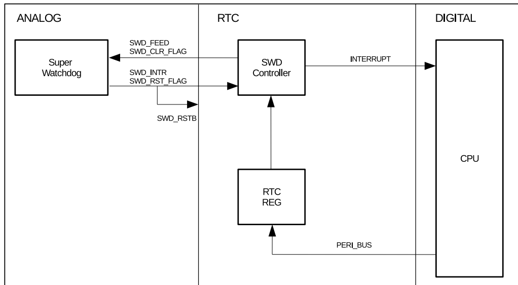
Figure 11.3-1. Super Watchdog Controller Structure
