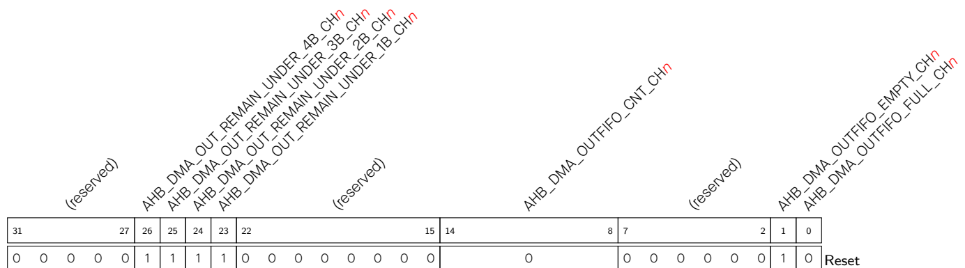
Register 3.37. AHB_DMA_OUTFIFO_STATUS_CH n _REG ( n : 0-2) (0x00D8+0xC0* n )
