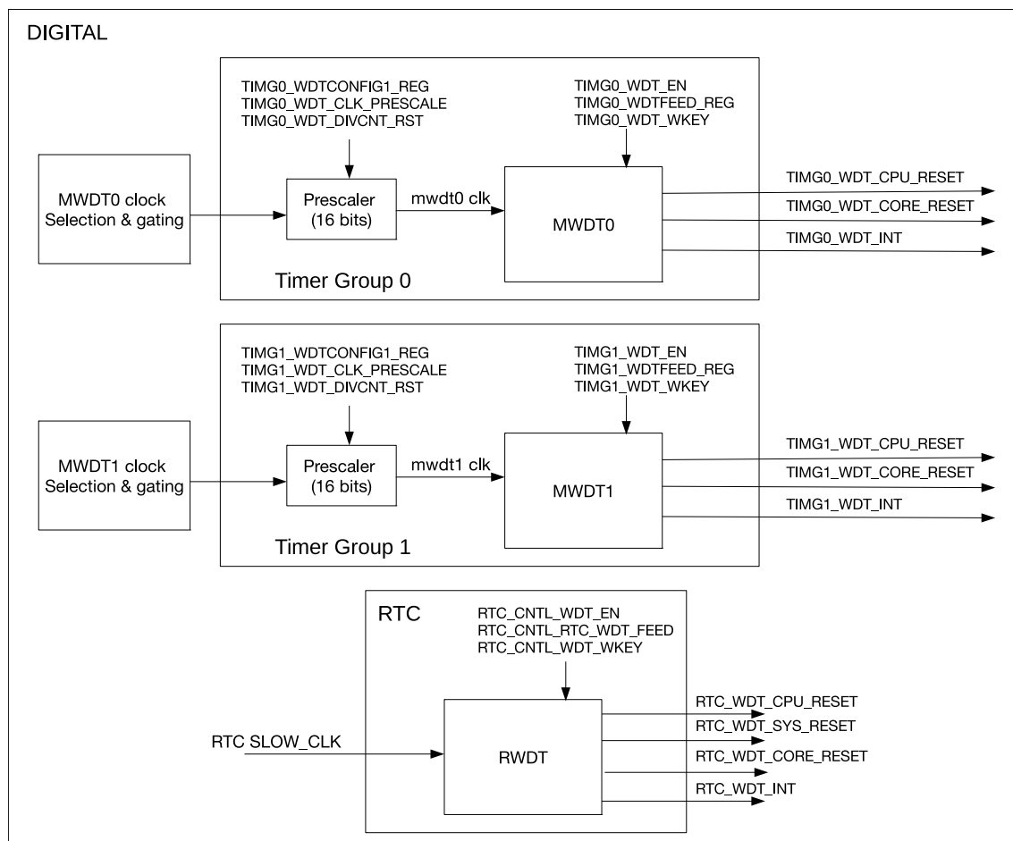
Figure 11.2-1. Digital Watchdog Timers in ESP32-C5
