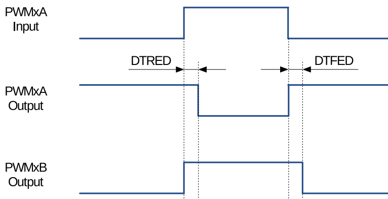
Figure 31.3-23. Active Low Complementary (ALC) Dead Time Waveforms
