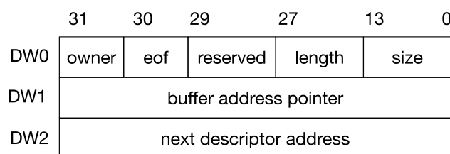
Figure 29.5-5. DMA Linked List Descriptor Structure of the SDIO Slave
