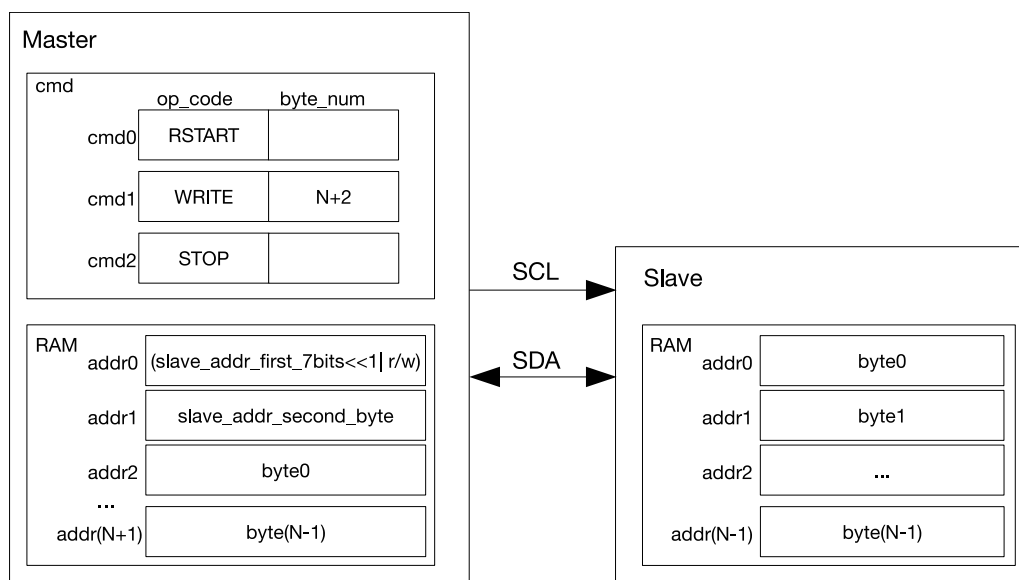
Figure 26.7-2. I2C master Writing to a Slave with a 10-bit Address
