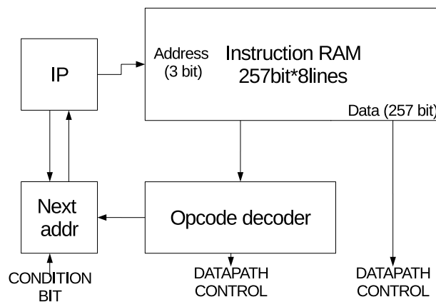
Figure 34.4-2. BitScrambler Control Path Diagram
