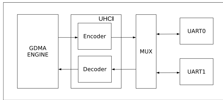
Figure 25.4-10. Data Transfer in GDMA Mode
