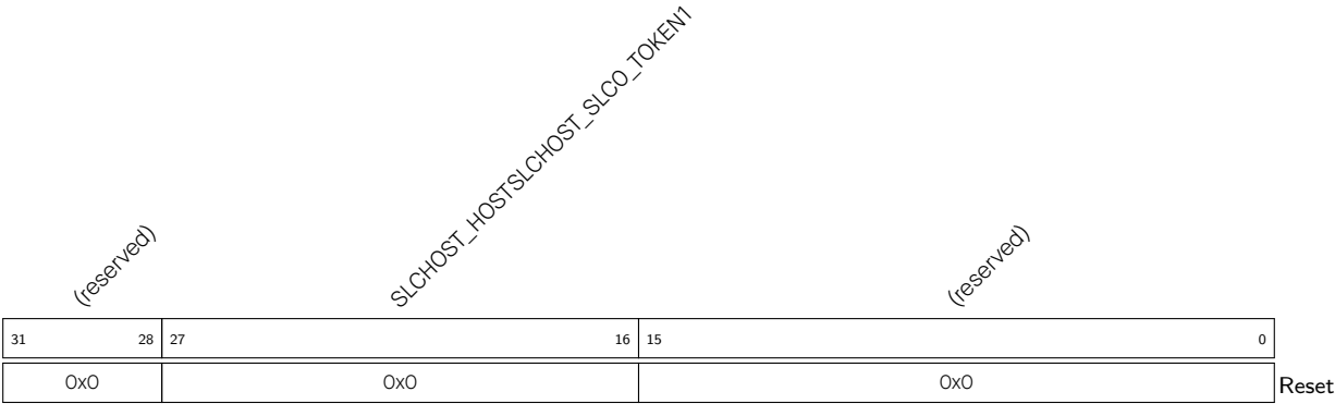
Register 29.50. SLCHOST_SLC0HOST_TOKEN_RDATA_REG (0x0044)
