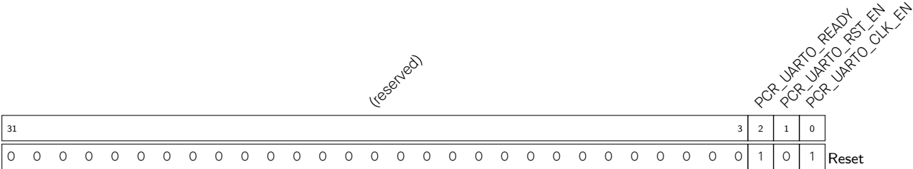
Register 6.1. PCR_UARTO_CONF_REG (0x0000)
