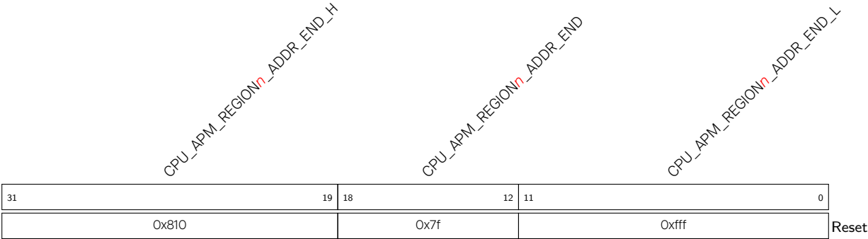
Register 13.59. CPU_APM_REGION n _ADDR_END_REG ( n : 0-7) (0x0008+0xC* n )
