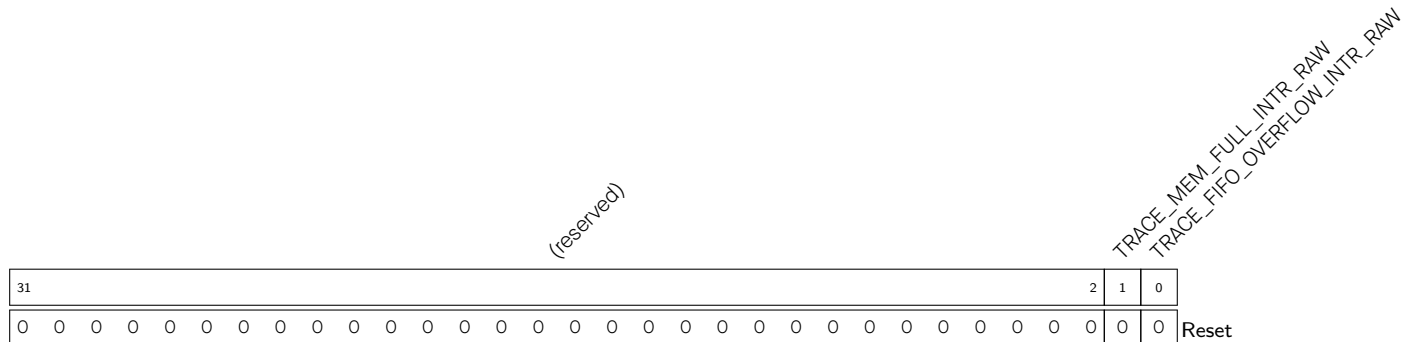
Register 1.7. TRACE_INTR_RAW_REG (0x0018)
