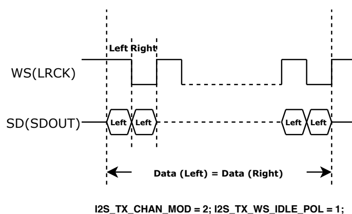
Figure 27.9-3. PDM Channel Control Example
