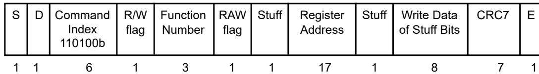
Figure 29.5-1. CMD52 Content
