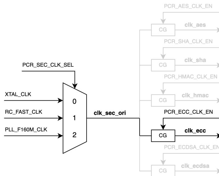
Figure 17.4-1. clk_ecc Diagram
