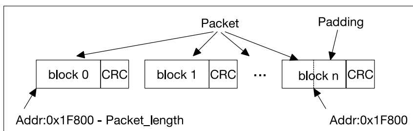
Figure 29.5-7. Data Flow of Sending Incremental-address Packets From Host to Slave
