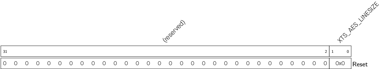
Register 23.2. XTS_AES_LINESIZE_REG (0x0340)
