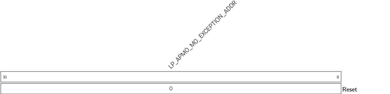
Register 13.53. LP_APMO_MO_EXCEPTION_INFO1_REG (0x00D4)
