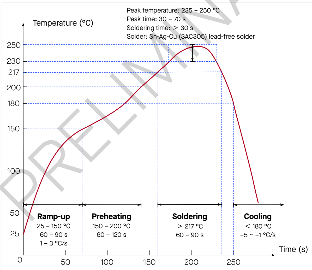
Figure 15: Reflow Profile
