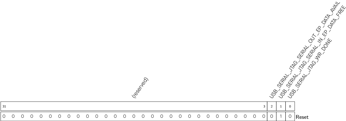
Register 26.2. USB_SERIAL_JTAG_EP1_CONF_REG (0x0004)
