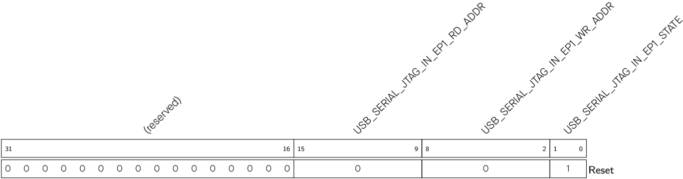
Register 26.21. USB_SERIAL_JTAG_IN_EP1_ST_REG (0x002C)
