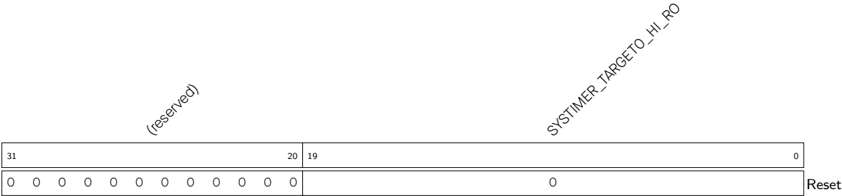
Register 10.31. SYSTIMER_REAL_TARGET0_HI_REG (0x0078)
