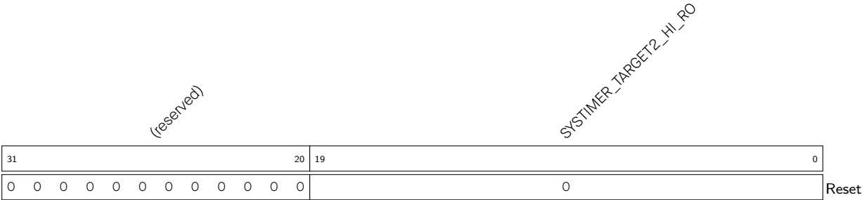
Register 10.35. SYSTIMER_REAL_TARGET2_HI_REG (0x0088)
