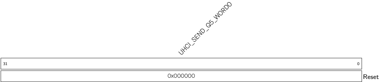
Register 22.54. UHCI_REG_Q5_WORD0_REG (0x005C)
