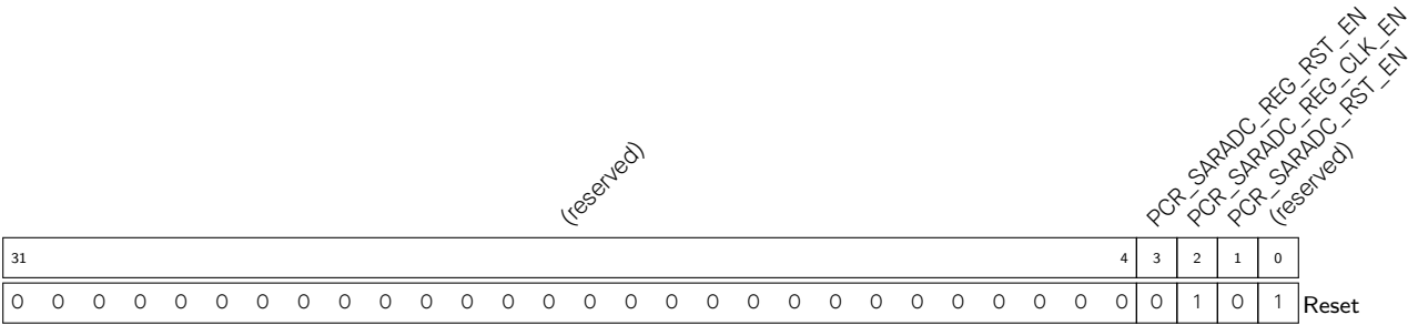
Register 5.28. PCR_SARADC_CONF_REG (0x0074)
