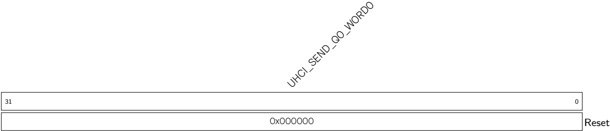
Register 22.44. UHCI_REG_Q0_WORD0_REG (0x0034)
