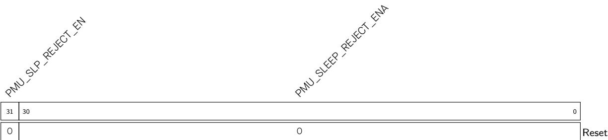
Register 9.71. PMU_SLP_WAKEUP_CNTL1_REG (0x0128)
