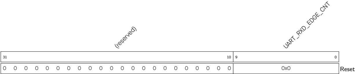
Register 22.34. UART_RXD_CNT_REG (0x0084)
