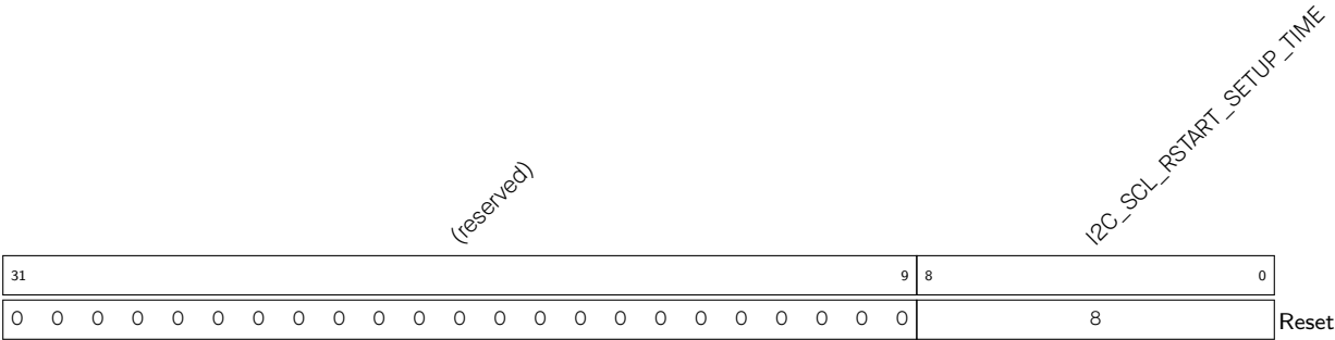
Register 24.6. I2C_SCL_RSTART_SETUP_REG (0x0044)
