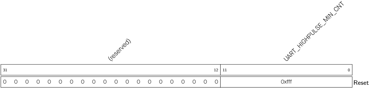
Register 22.33. UART_HIGHPULSE_REG (0x0080)
