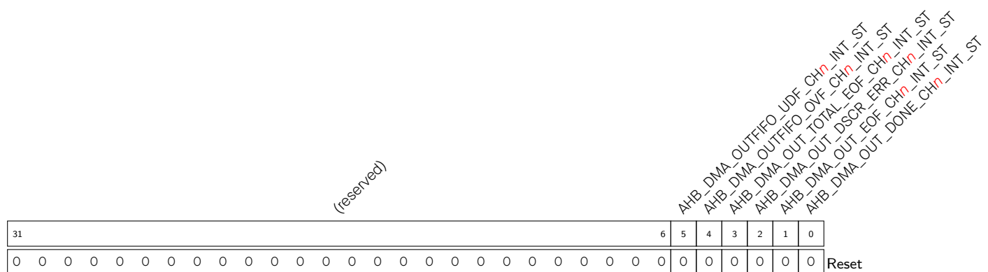
Register 2.6. AHB_DMA_OUT_INT_ST_CH n _REG ( n : 0-1) (0x0034+0x10* n )
