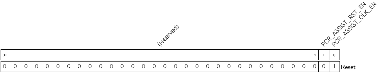
Register 5.50. PCR_ASSIST_CONF_REG (0x00D4)
