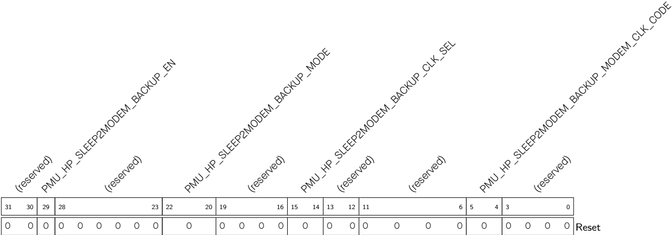
Register 9.21. PMU_HP_MODEM_BACKUP_REG (0x0050)
