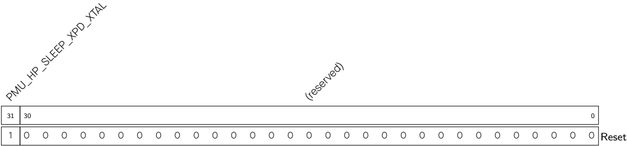
Register 9.39. PMU_HP_SLEEP_XTAL_REG (0x0098)
