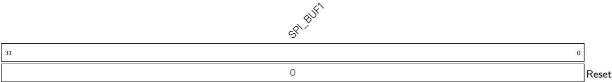
Register 23.23. SPI_W1_REG (0x009C)
