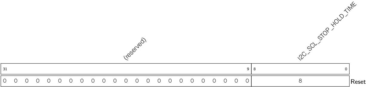
Register 24.7. I2C_SCL_STOP_HOLD_REG (0x0048)
