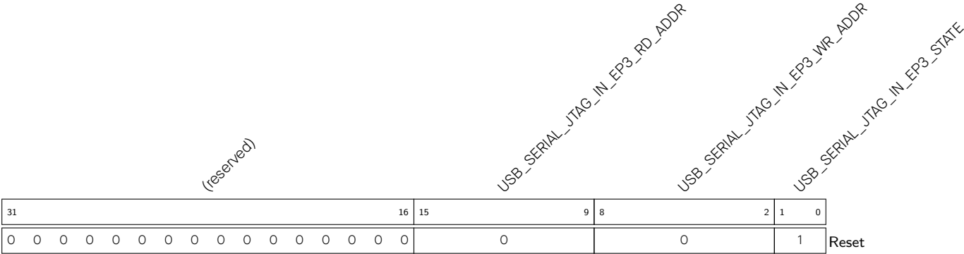
Register 26.23. USB_SERIAL_JTAG_IN_EP3_ST_REG (0x0034)
