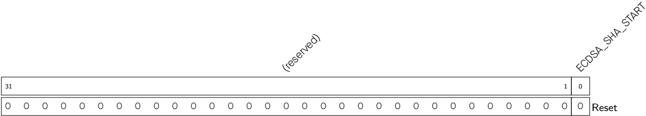
Register 19.11. ECDSA_SHA_START_REG (0x0210)
