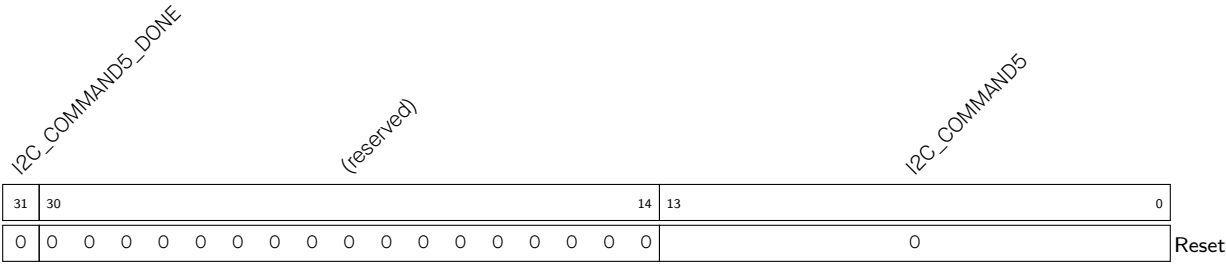
Register 24.30. I2C_COMD5_REG (0x006C)
