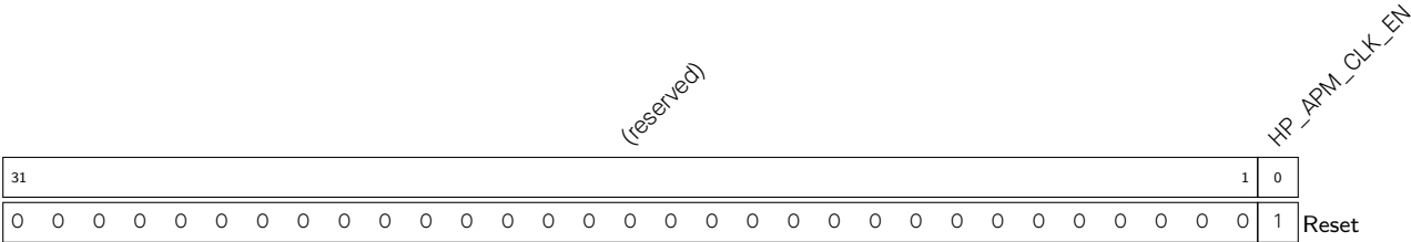
Register 14.23. HP_APM_CLOCK_GATE_REG (0x07F8)
