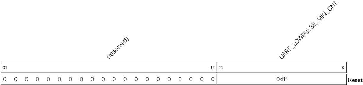
Register 22.32. UART_LOWPULSE_REG (0x007C)
