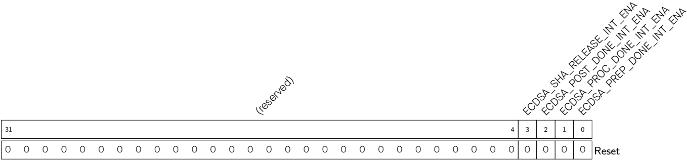
Register 19.6. ECDSA_INT_ENA_REG (0x0014)
