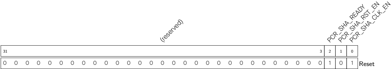
Register 5.37. PCR_SHA_CONF_REG (0x00A0)
