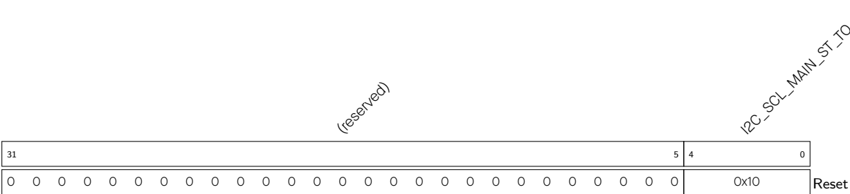
Register 24.10. I2C_SCL_MAIN_ST_TIME_OUT_REG (0x007C)
