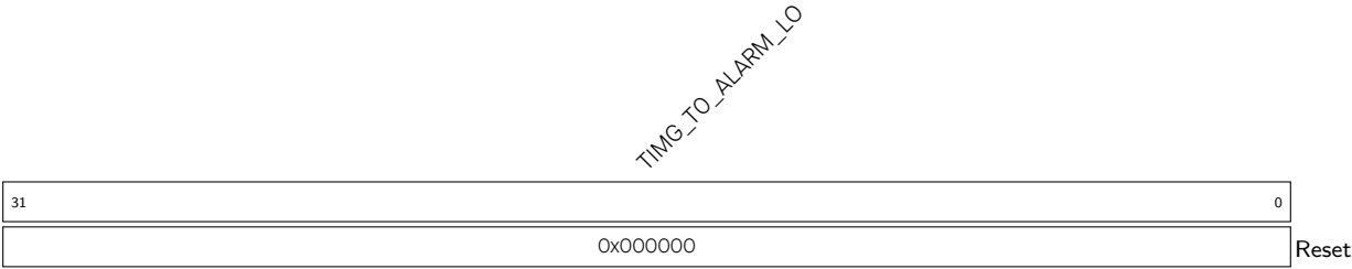
Register 11.5. TIMG_TOALARMLO_REG (0x0010)
