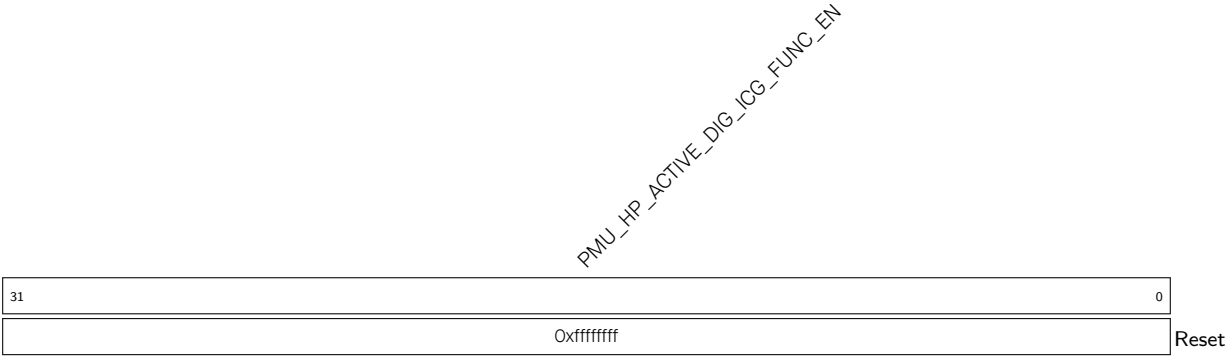
Register 9.2. PMU_HP_ACTIVE_ICG_HP_FUNC_REG (0x0004)
