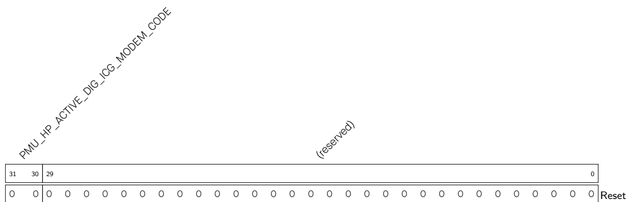
Register 9.4. PMU_HP_ACTIVE_ICG_MODEM_REG (0x000C)
