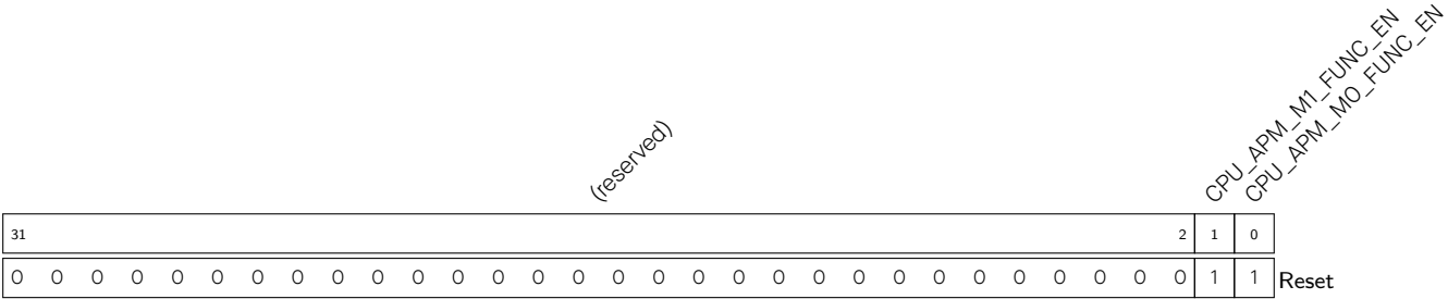
Register 14.41. CPU_APM_FUNC_CTRL_REG (0x00C4)
