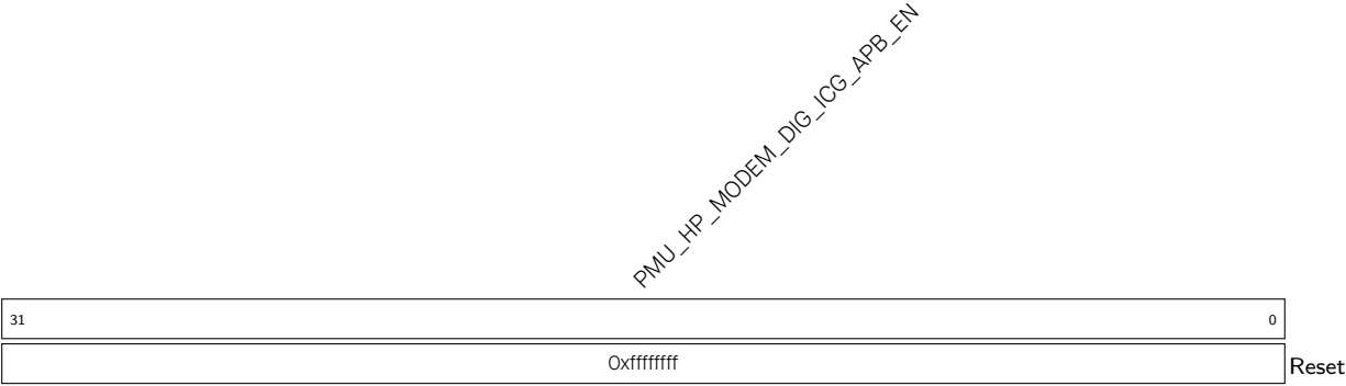
Register 9.16. PMU_HP_MODEM_ICG_HP_APB_REG (0x003C)
