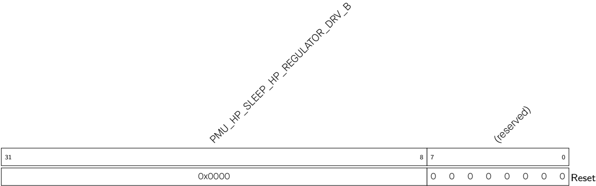
Register 9.38. PMU_HP_SLEEP_HP_REGULATOR1_REG (0x0094)
