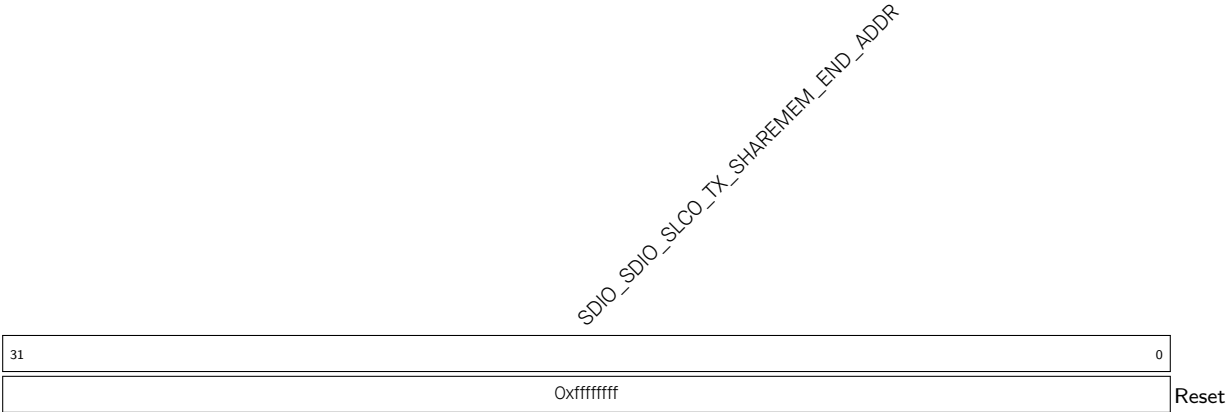
Register 27.22. SDIO_SLC0_TX_SHAREMEM_END_REG (0x0158)
