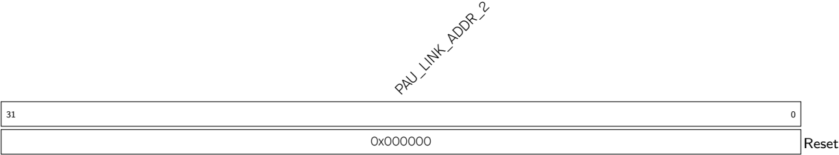
Register 9.98. PAU_REGDMA_LINK_2_ADDR_REG (0x0014)
