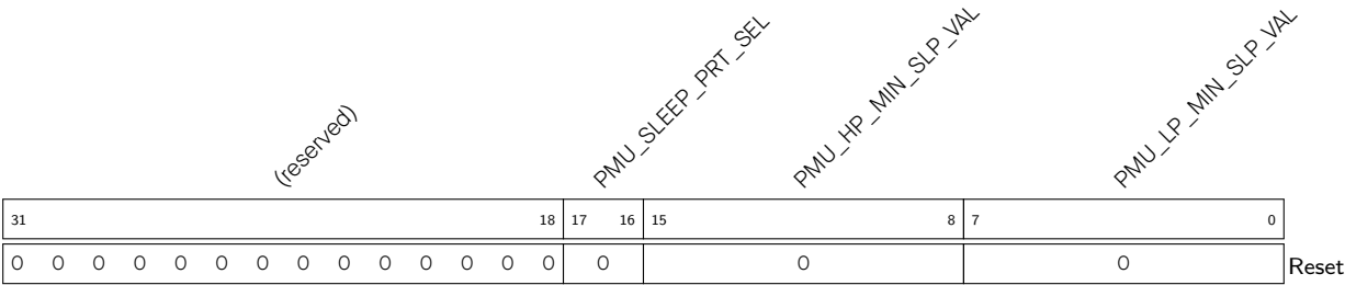
Register 9.73. PMU_SLP_WAKEUP_CNTL3_REG (0x0130)
