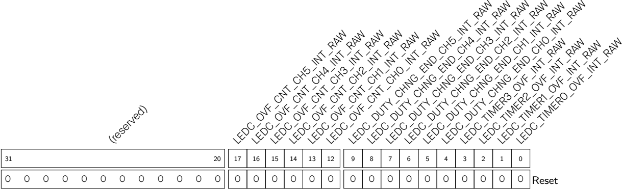
Register 28.15. LEDC_INT_RAW_REG (0x00C0)
