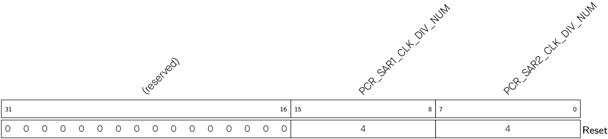
Register 5.63. PCR_SAR_CLK_DIV_REG (0x0124)
