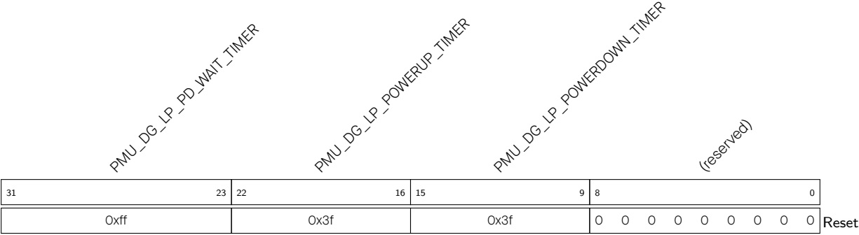
Register 9.58. PMU_POWER_WAIT_TIMER1_REG (0x00F0)
