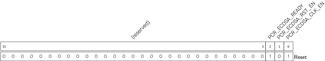
Register 5.44. PCR_ECDSA_CONF_REG (0x00BC)
