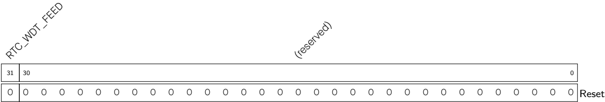
Register 12.6. RTC_WDT_FEED_REG (0x0014)
