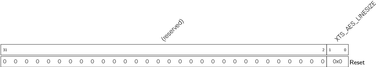
Register 20.2. XTS_AES_LINESIZE_REG (0x0340)
