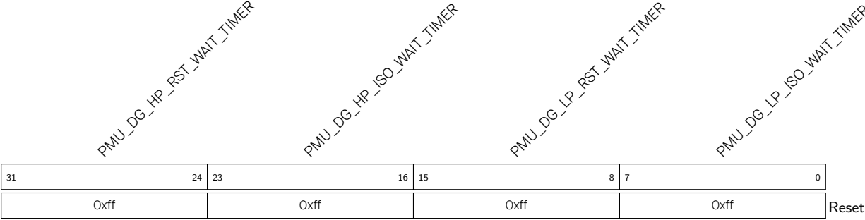
Register 9.59. PMU_POWER_WAIT_TIMER2_REG (0x00F4)
