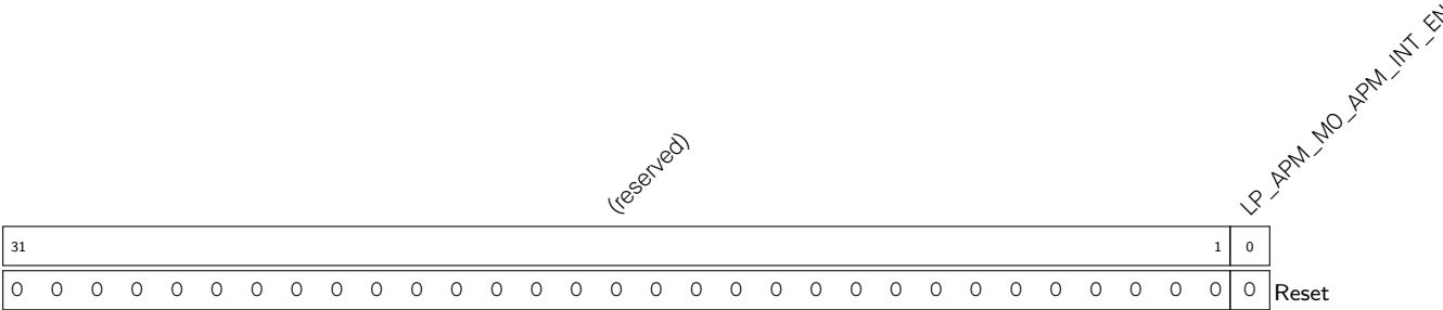
Register 14.34. LP_APM_INT_EN_REG (0x00E8)
