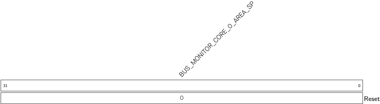
Register 15.26. BUS_MONITOR_CORE_0_AREA_SP_REG (0x0034)
