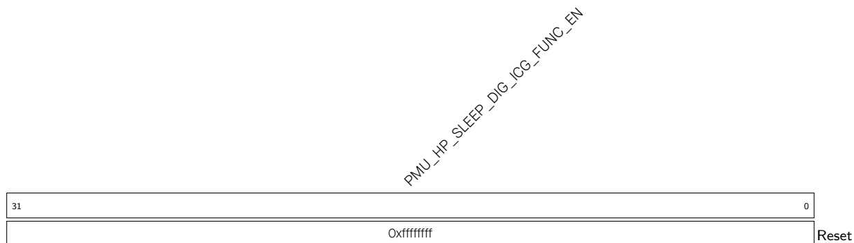
Register 9.28. PMU_HP_SLEEP_ICG_HP_FUNC_REG (0x006C)
